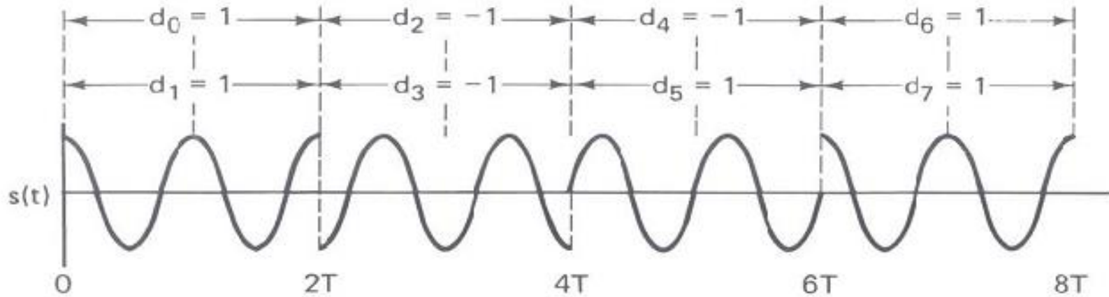
(a) QPSK
