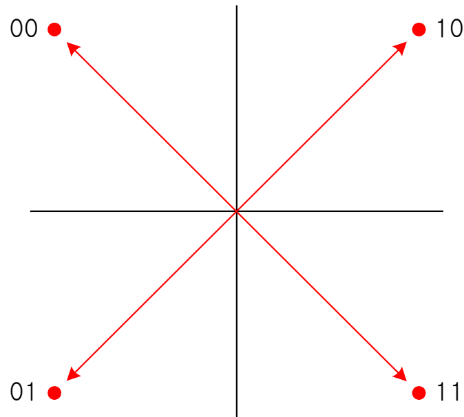
(a) QPSK
