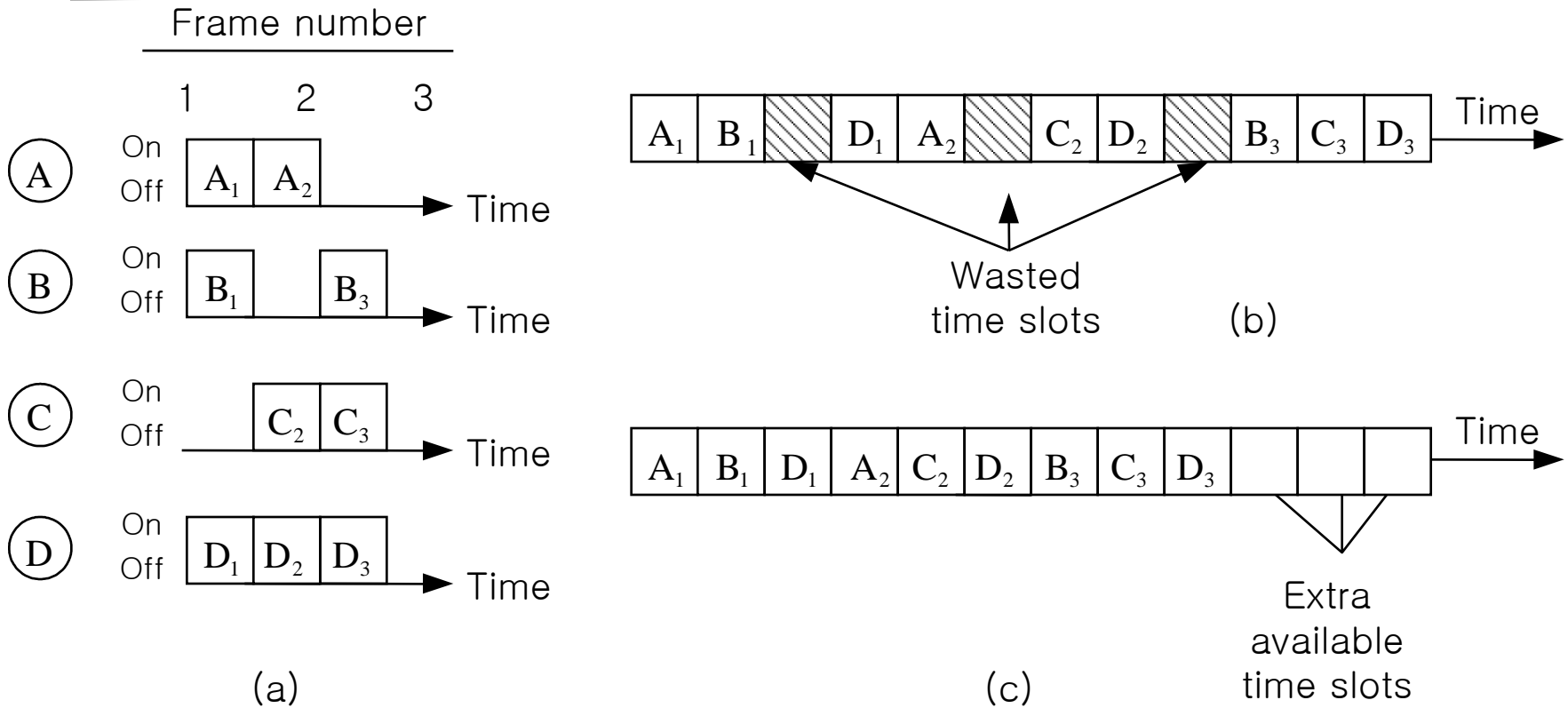
Fixed-assignment TDM versus packet switching. (a) Data source activity profiles. (b) Fixed-assignment time-assignment time-division multiplexing. (c) Time-division packet switching (concentration)
