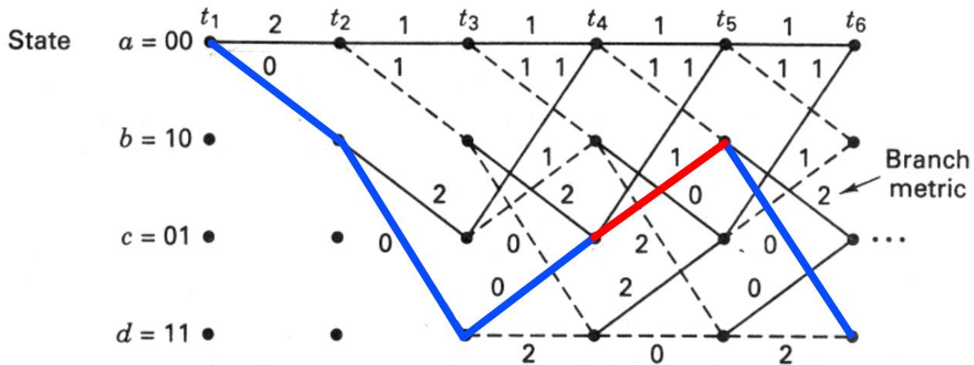
Figure 7.10 Decoder trellis diagram (rate \frac{1}{2} , K = 3 ).
