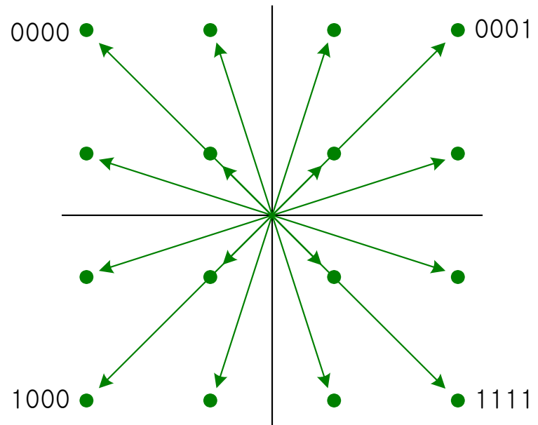
(a) QAM
